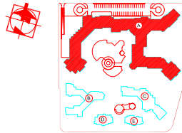
BUILDING - A FLOOR 2, LEVEL +3.60 M1:200
